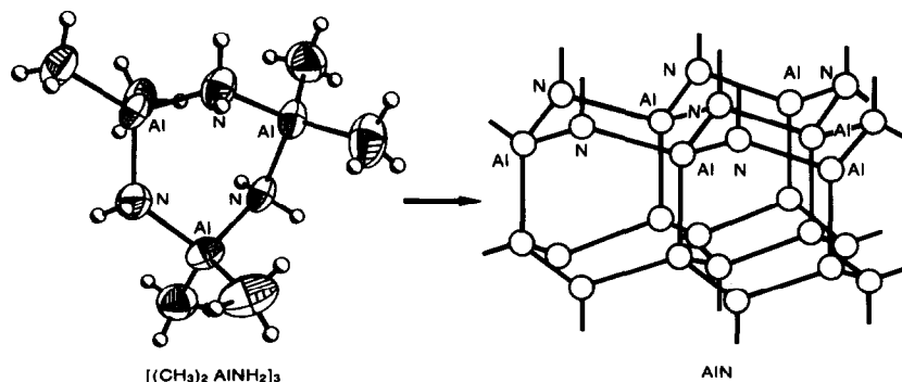
Fig. 3. Structural relationship between [\text{Me}_2\text{AlNH}_2]_3 and AlN.
