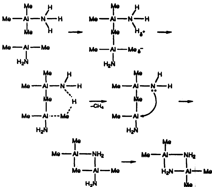
Scheme 3. Proposed mechanism for the thermal decomposition of \text{Me}_3\text{Al}:\text{NH}_3 .
