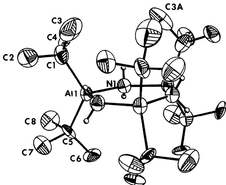
Fig. 2. Ortep plot of (t\text{-Bu}_2\text{AlNH}_2)_3 . Hydrogen atoms omitted (except on N) for clarity.
